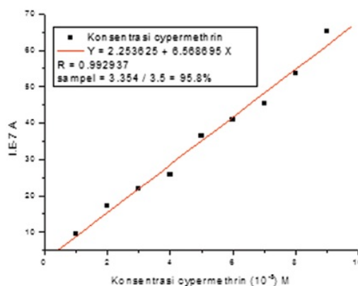
Fig. 3. DPV voltammograms and standard addition curve of cypermethrin of agricultural soil samples from Distric Pace, Nganjuk East Java.
