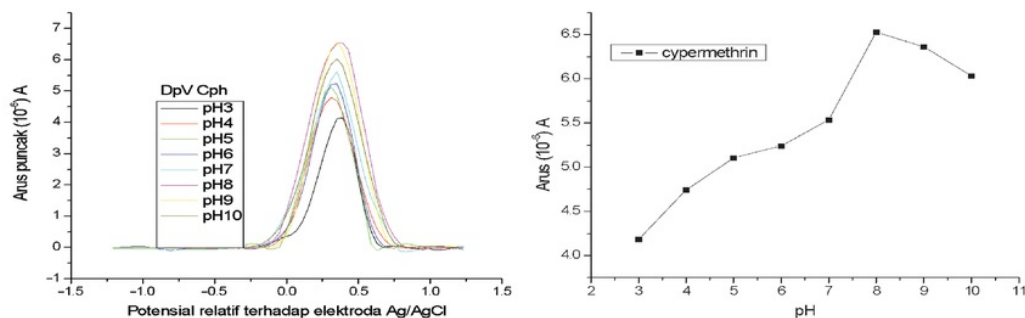
Fig. 1. Voltammogram of DPV of 10^{-5} M cypermethrin to the pH (3–10).
