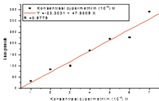
Fig. 5. Standard curve of cypermethrin.
